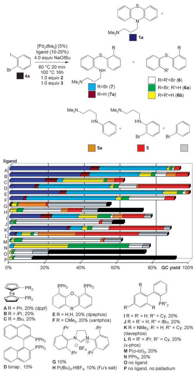
Figure 1. Ligand screening. Reactions were performed on 0.26-mmol scale using 5% [Pd 2 dba 3 ] and 10–20% ligand in toluene (2 mL). The colors in the chart indicate the product distribution across the range of ligands (A–N) studied in addition to two control experiments (O and P). Cy = cyclohexyl; tol = tolyl.
